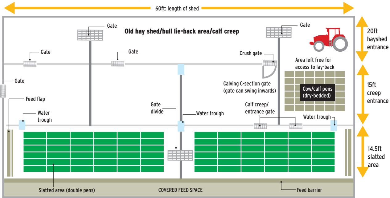
Multipurpose slatted shed combined with existing hay shed
