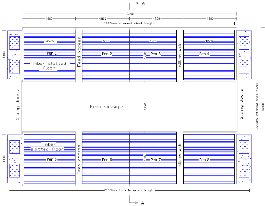
Plan view - 4 bay slatted sheep house
