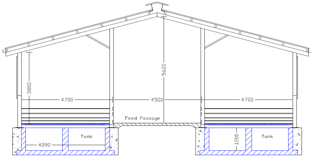
Section AA - slatted sheep house
