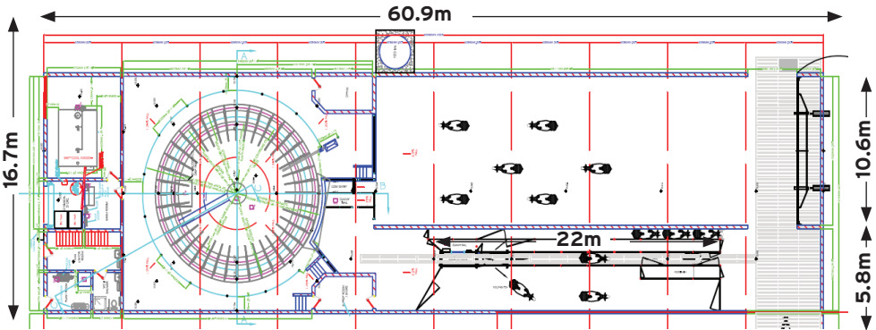
Figure 1: Plan view of rotary parlour, collecting yard and drafting area.
